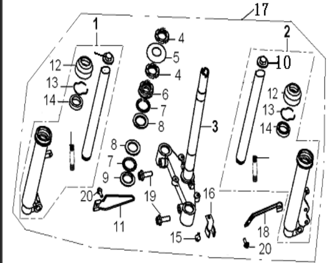
F03 Front fork
