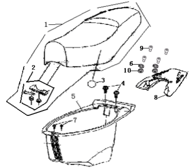
F09 Seat
