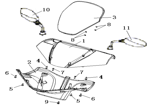
F15Handle cover
