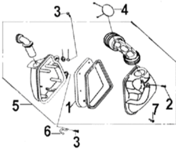
F07 Air cleaner
