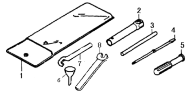
F23 Tool kit
