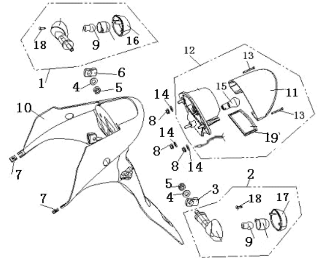
F20 Tail light
