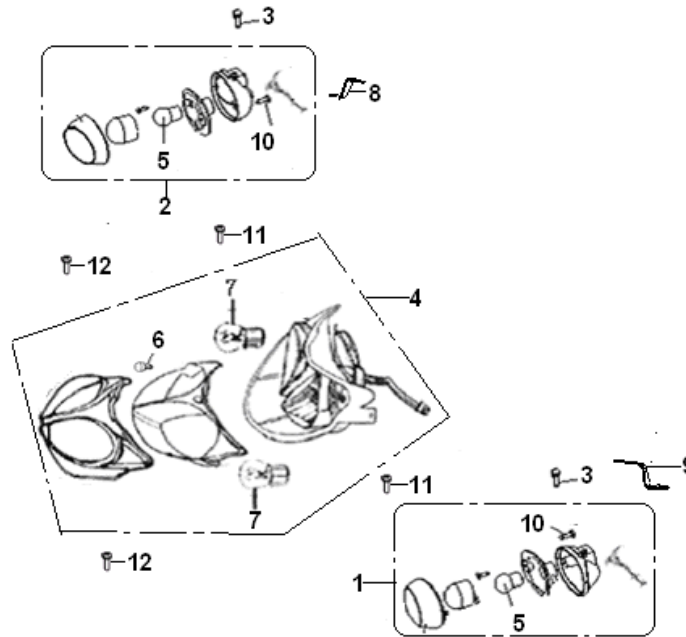
F22 Electrical equipment 1
