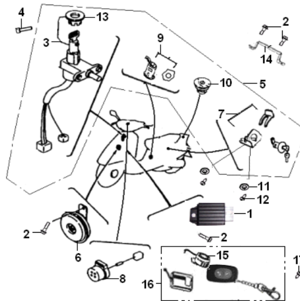
F22 Electrical equipment 1
