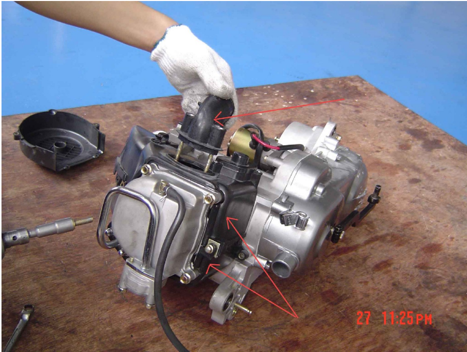
Fig. 16. Install carb inlet tube.
