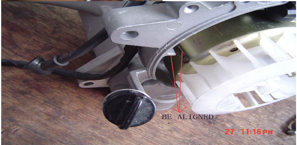
Fig 7. a & b. Install the cylinder head. Rotate the magneto and chain until the markings are lined up.
