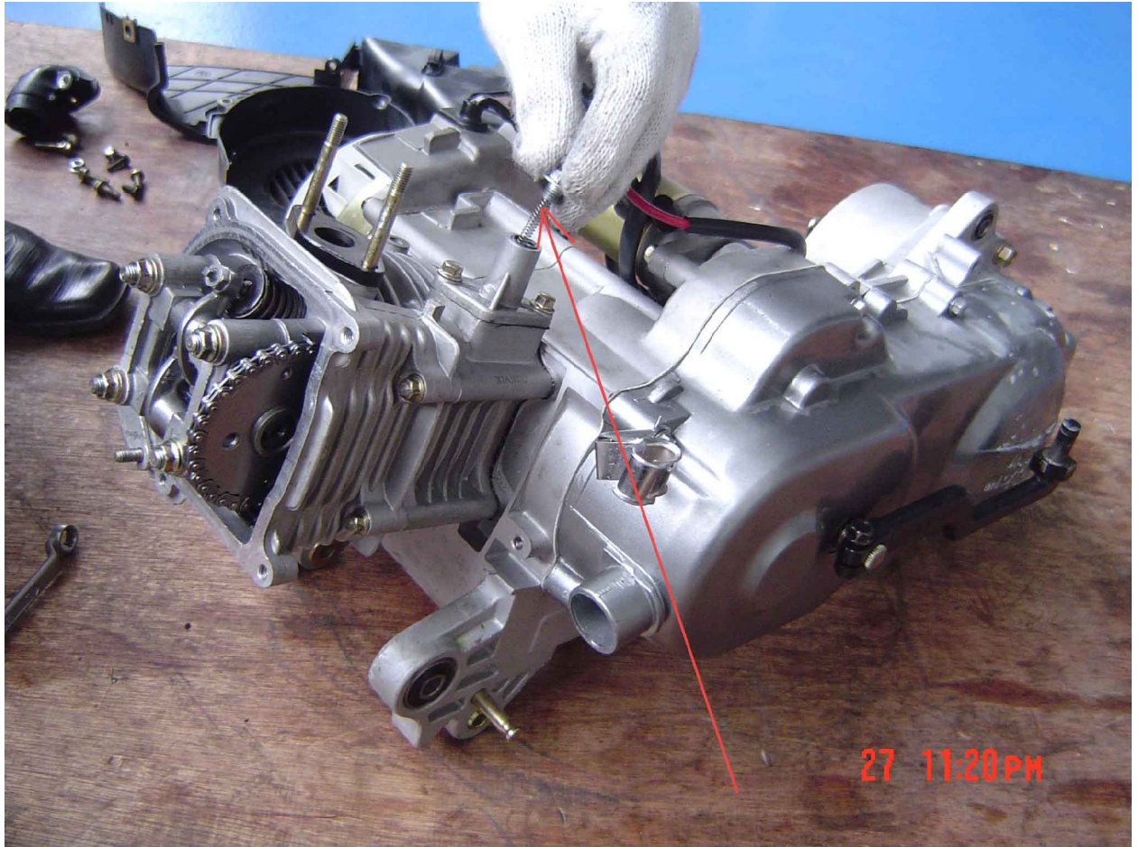
Fig. 12b. Install chain tension.
